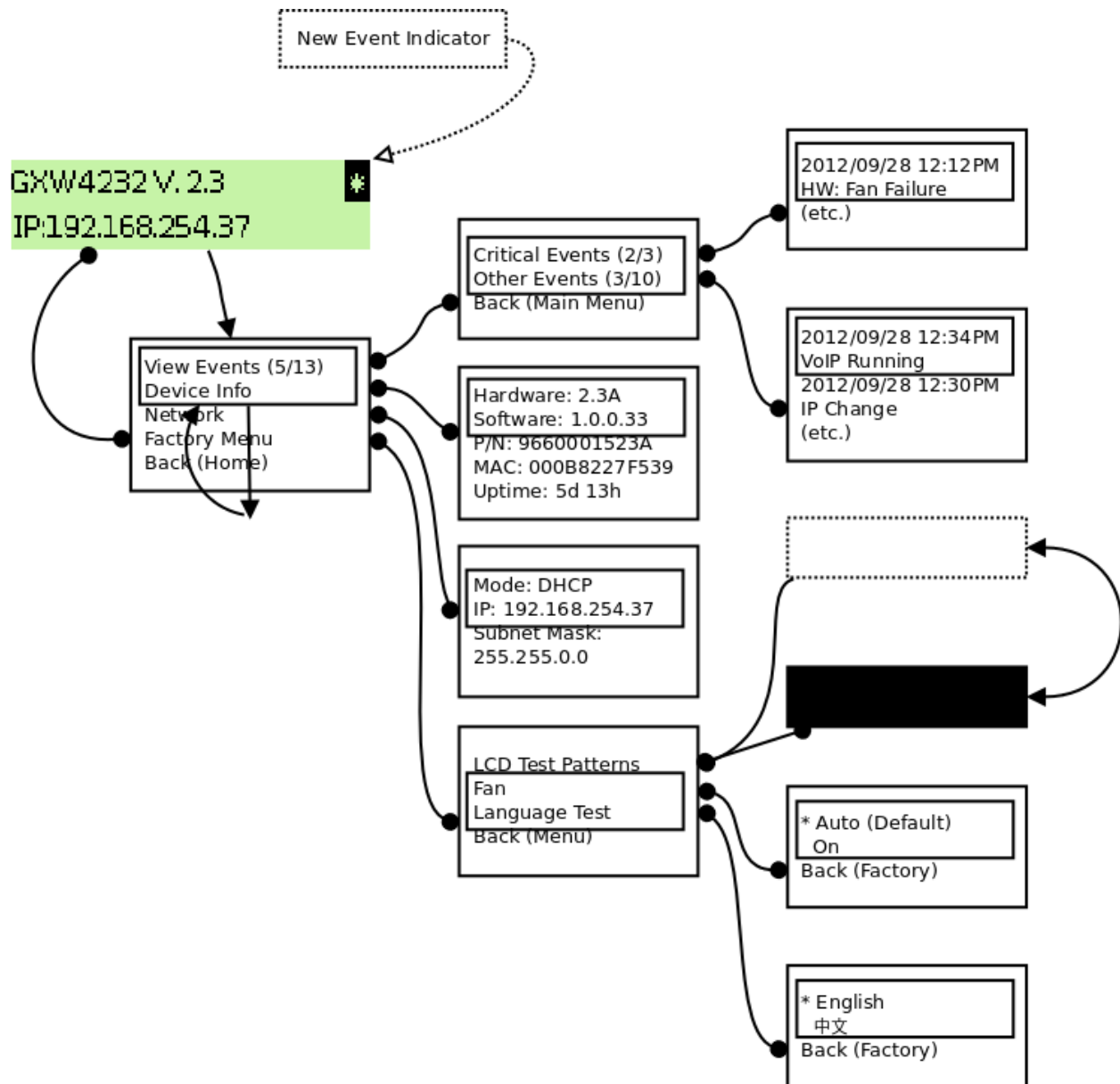
FIGURE 3: LCD MENU
